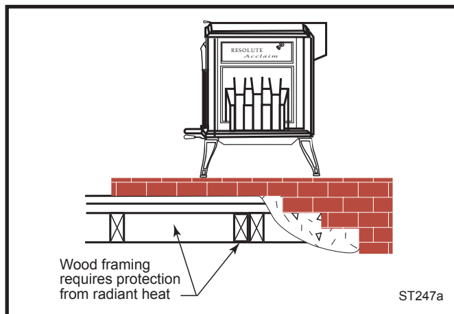
Fig. 12 Supporting timbers under fireplace hearth are considered to be combustible
